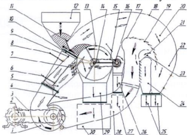
Figure 1. Technological scheme of pneumatic separator
