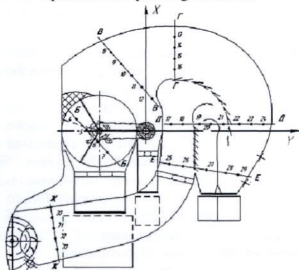
Figure 3 - Scheme of the laboratory-production plant for removing the characteristics of the air flow in the zone of the sedimentary chamber.
