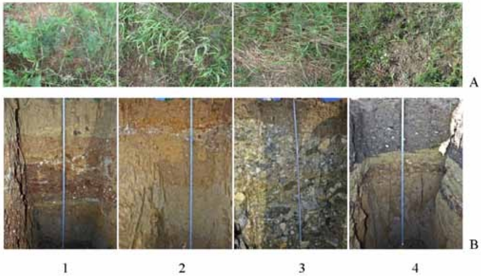
Fig. 2. Plant cover (A) and soil section of the test polygons. Notes: 1 – technosols on loess-like loams; 2. – technosols on red-brown clays; 3. – technosols on gray-green clays; 4. – technosols on humus-rich layer (pedozem).
