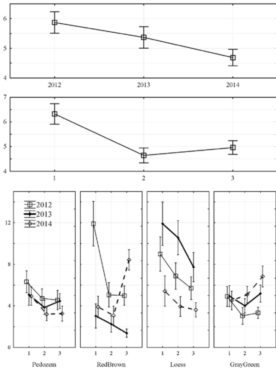
Fig. 5. Dynamics of the Chondrula tridens population abundance in different technosol types (ind./m 2 , mean \pm 95% confidence interval).
